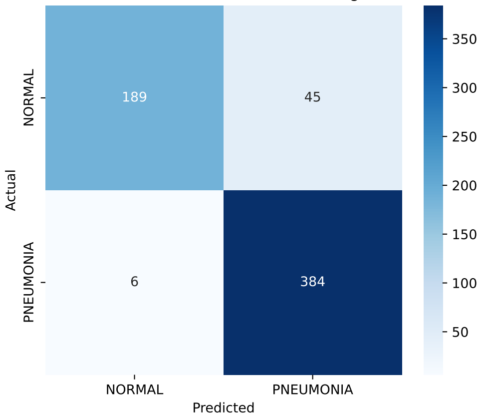
Confusion Matrix - Full Fine-Tuning
